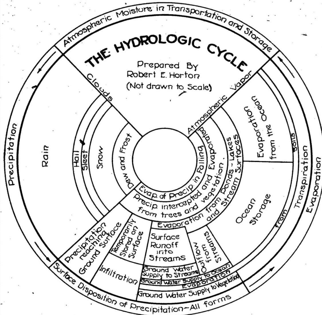
Fig. 1--The hydrologic cycle
